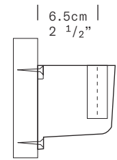
WALL BRACKET B-LARGE
